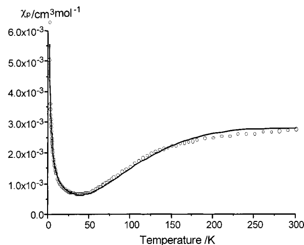
Figure 3. The molar susceptibility of 1 per unit dimer as a function of temperature (circles = experimental values, solid line = calculated for J = -92 \text{ cm}^{-1} )
