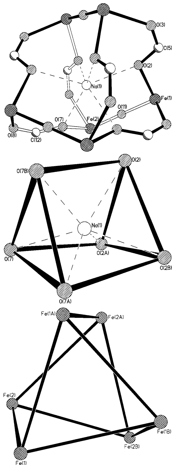
Figure 2. a) The central core of 1 ; b) the coordination environment of the Na + cation; c) the distorted trigonal prismatic arrangement of the iron atoms
