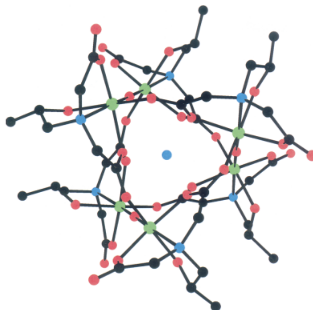
Figure 1. The cation of [\text{Fe}_6(\text{C}_7\text{H}_{11}\text{NO}_5)_6(\mu_2\text{-O})_3\text{Na}]^+ ( 1 ) viewed down the a axis
